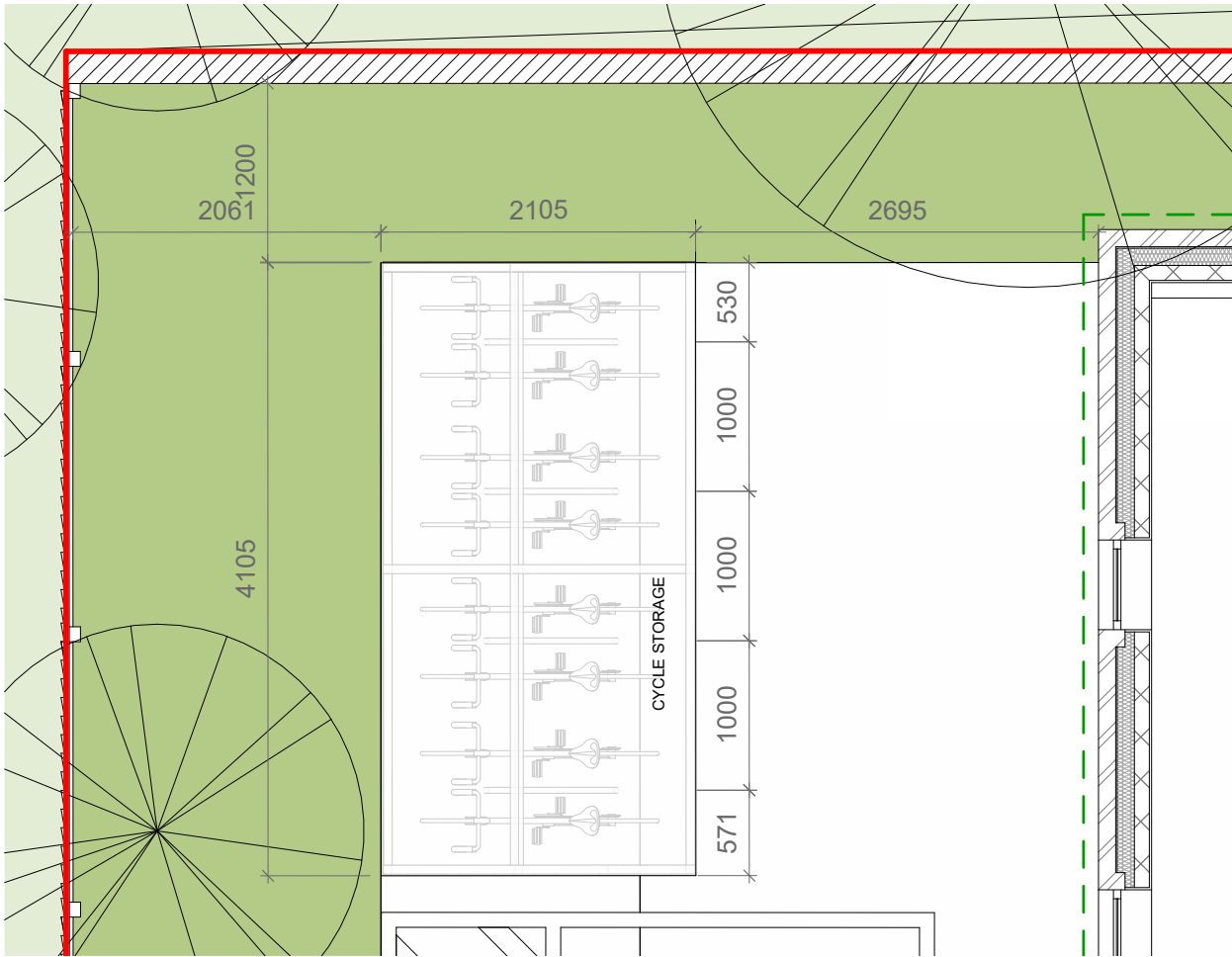
1 Proposed Site Layout Plan 1 : 50
