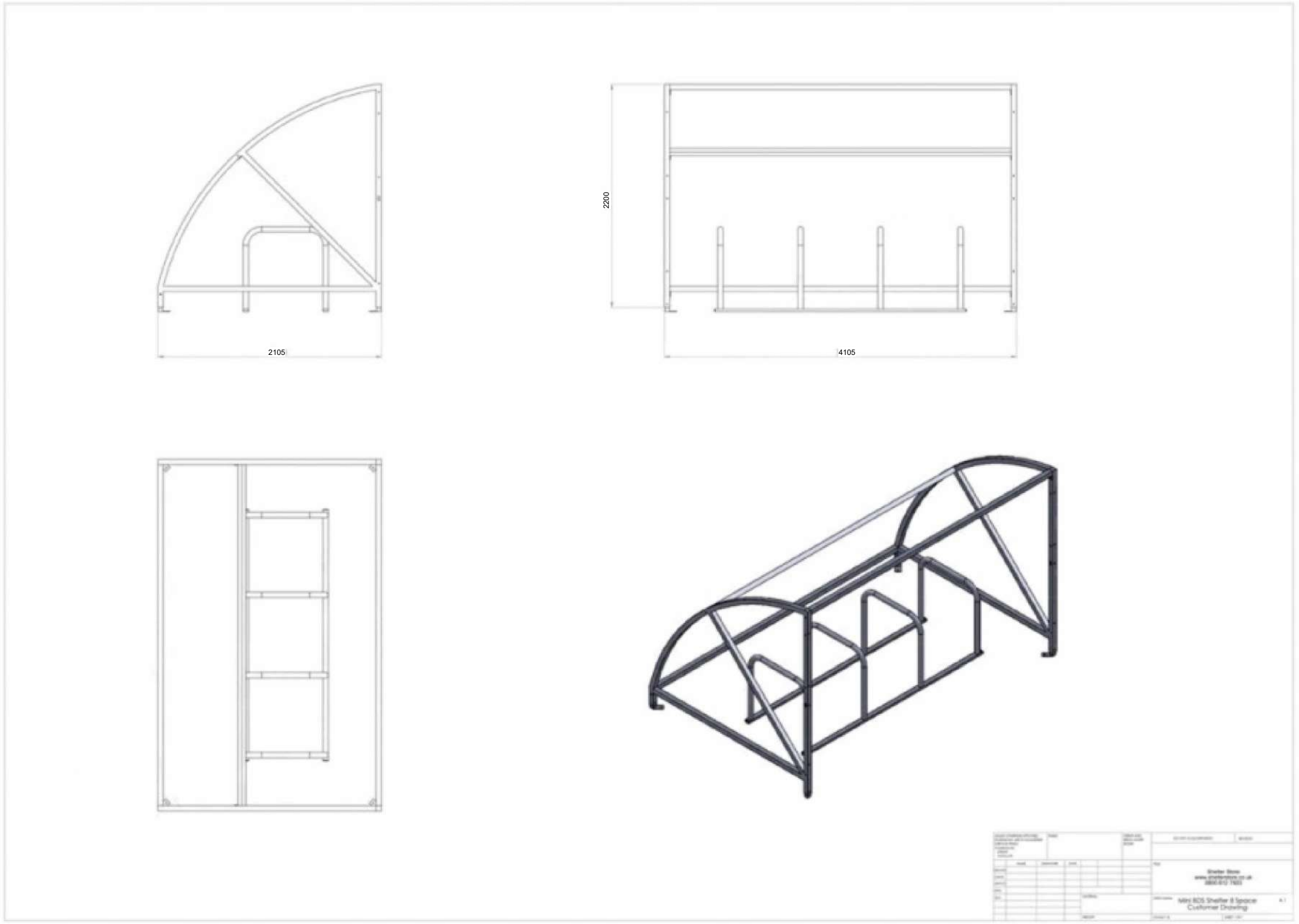
Bike shelter and stand setting out
