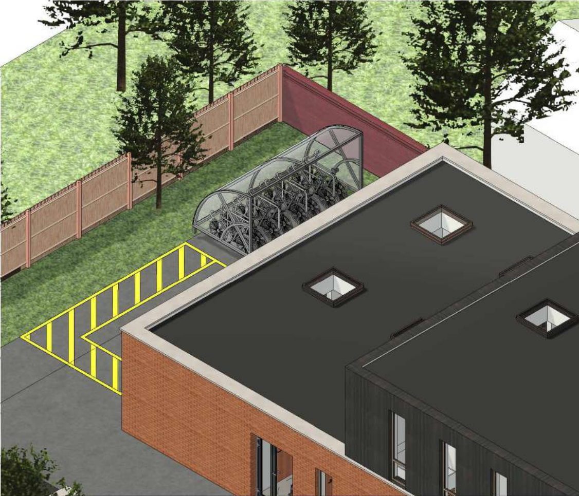
2 CYCLE STORAGE - 3D VIEW 01
